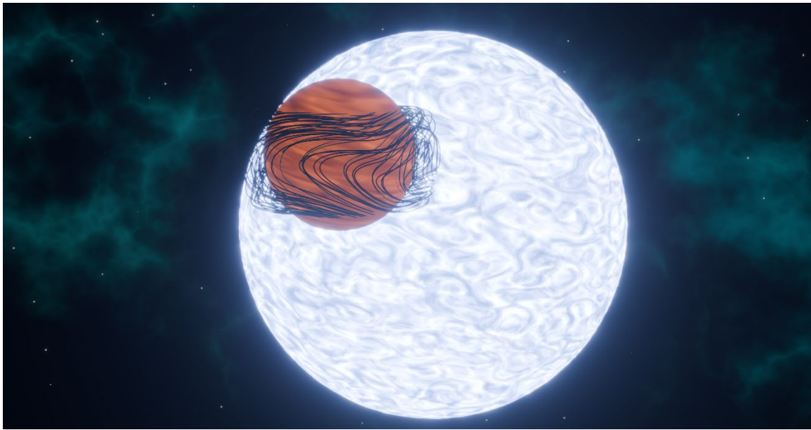
Artist's rendering of the gas giant KELT-9b, the hottest known exoplanet, passing in front of its star. The dark lines represent the planet's possible magnetic field. The SPIRou spectropolarimeter at the Canada-France-Hawaii Telescope may have detected the signature of this field during a transit of the exoplanet in 2025, but did not detect it again in 2026. Credit: Jean Guislain (IRAP - University of Toulouse).
